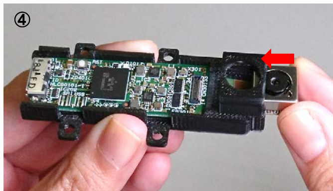
4. Hold the camera head and insert it horizontally. ! Be careful not to clash the board and the camera connector.
