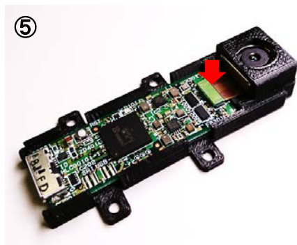
5. Combine the board and camera connector. ! Do not force down the connector.
