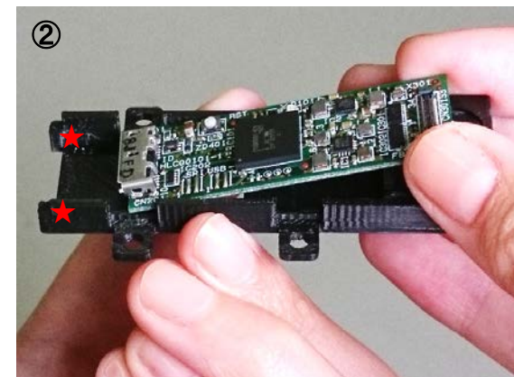
2. Insert the board into the slit of the part at an oblique angle. ★
