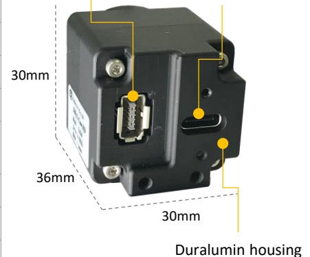
USB Type-C™ connector with lock screw
